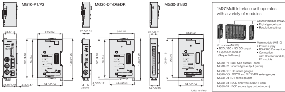
Interface unit
